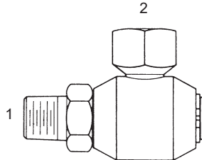
SLS-5502 - 90° (1) Male Pipe - Stem (2) Fem. Pipe - Barrel
