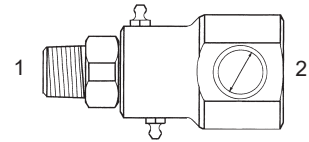
SLS-5502-SB-HP - 90° High Pressure - 10,000 PSI (1) Male Pipe - Stem (2) Fem. Pipe - Barrel (Short Body)
