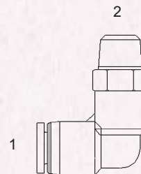
CPC-SB-2501-S - 90° (1) Tube (2) Male Pipe Swivel
