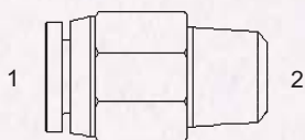
CPC-SB-2404 - Str. (1) Tube (2) Male Pipe
