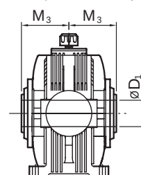
Hollow Output Shaft With Keyway - (K)
