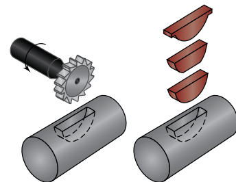
Woodruff Key
