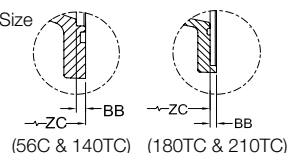
DETAIL C
