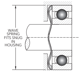
Gap-Type Wave Spring shown in a housing.
